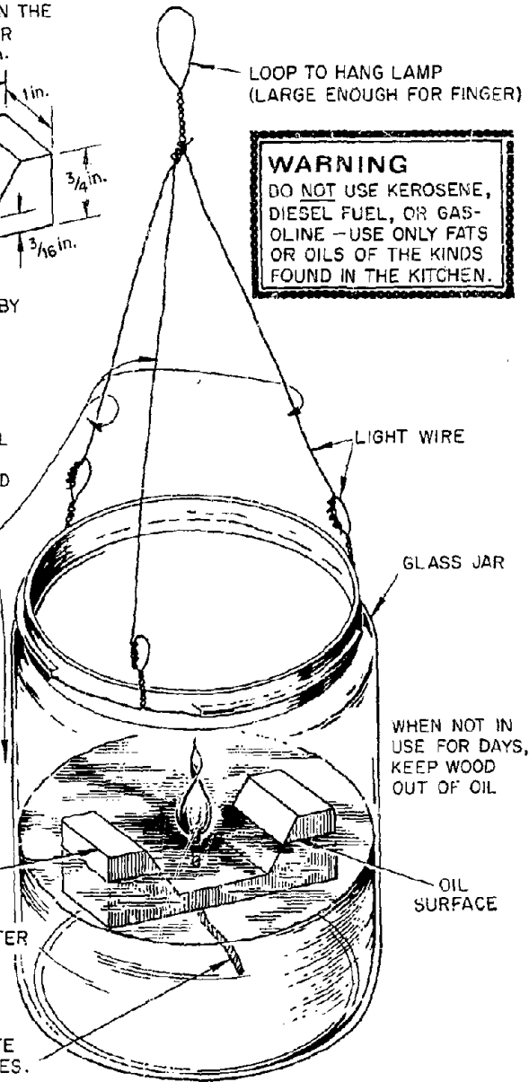
Fig. C-2. Floating Wick Lamp
